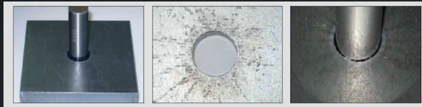
12 mm hole with True Hole Technology cut with HPRXD Plasma.
